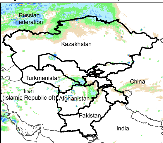
Daily Rainfall estimate for 23 Nov., 2015
