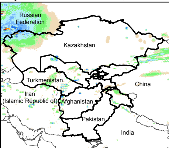
Daily Rainfall estimate for 24 Nov., 2015
