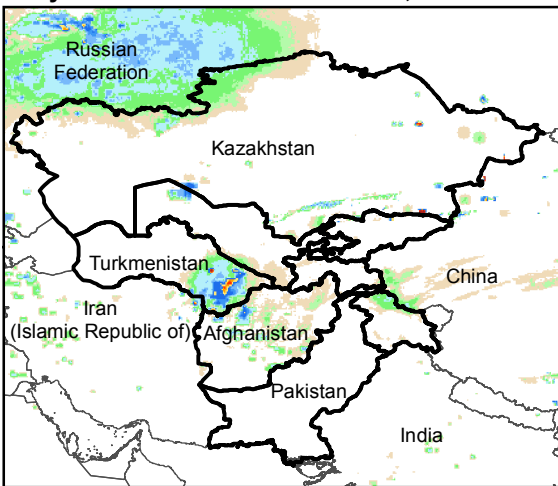
Daily Rainfall estimate for 25 Nov., 2015
