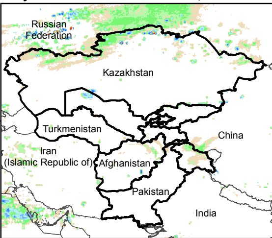
Daily Rainfall estimate for 27 Nov., 2015
