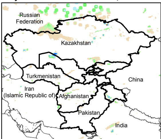
Daily Rainfall estimate for 28 Nov., 2015
