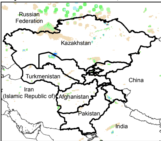
Daily Rainfall estimate for 1 Dec., 2015
