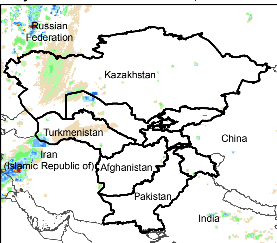
Daily Rainfall estimate for 2 Dec., 2015
