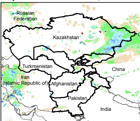
Daily Rainfall estimate for 6 Dec., 2015
