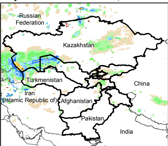
Daily Rainfall estimate for 4 Dec., 2015
