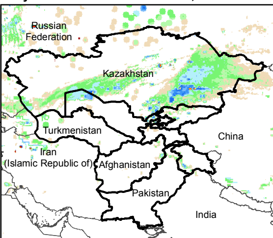
Daily Rainfall estimate for 5 Dec., 2015
