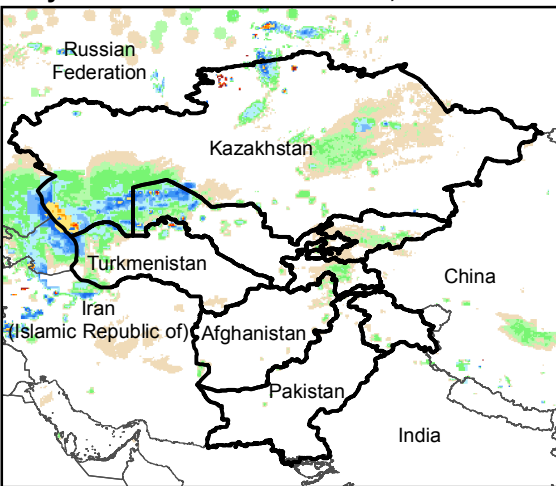
Daily Rainfall estimate for 7 Dec., 2015
