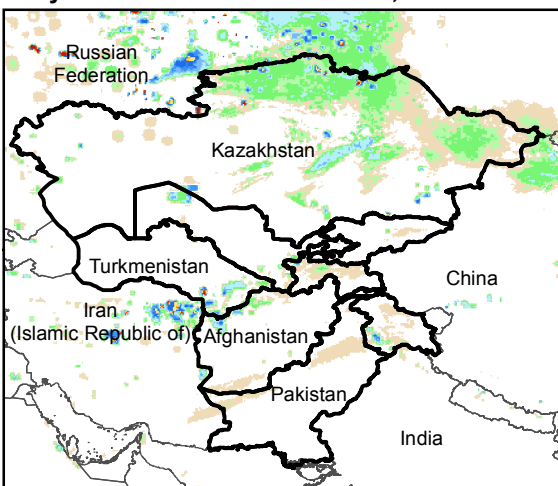
Daily Rainfall estimate for 8 Dec., 2015
