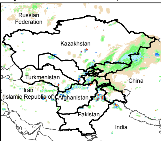
Daily Rainfall estimate for 10 Dec., 2015
