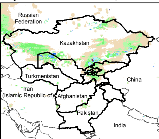
Daily Rainfall estimate for 19 Dec., 2015
