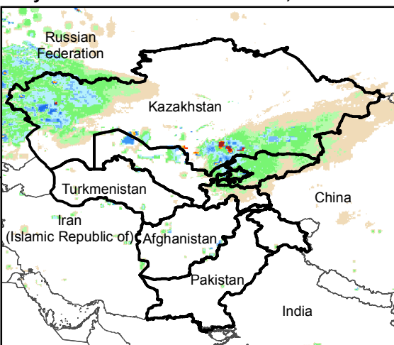
Daily Rainfall estimate for 20 Dec., 2015
