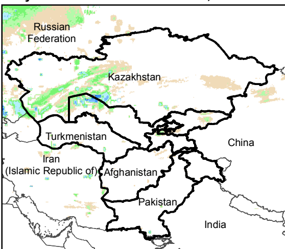
Daily Rainfall estimate for 21 Dec., 2015
