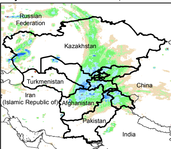
Daily Rainfall estimate for 4 Jan., 2016
