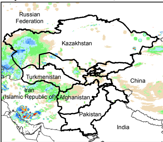
Daily Rainfall estimate for 5 Jan., 2016
