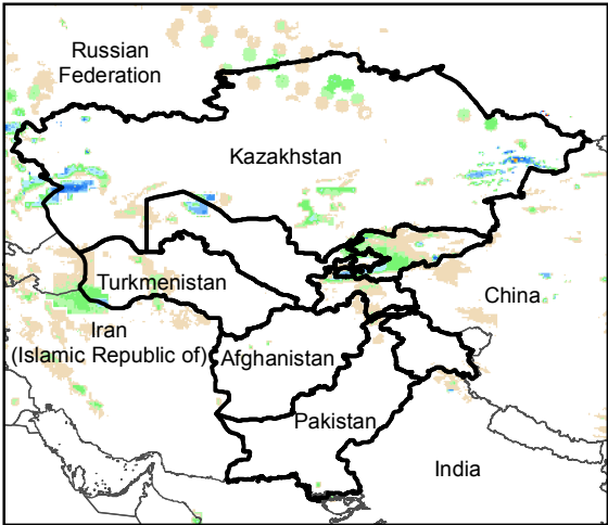
Daily Rainfall estimate for 6 Jan., 2016
