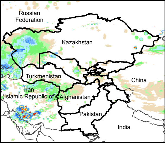
Daily Rainfall estimate for 5 Jan., 2016
