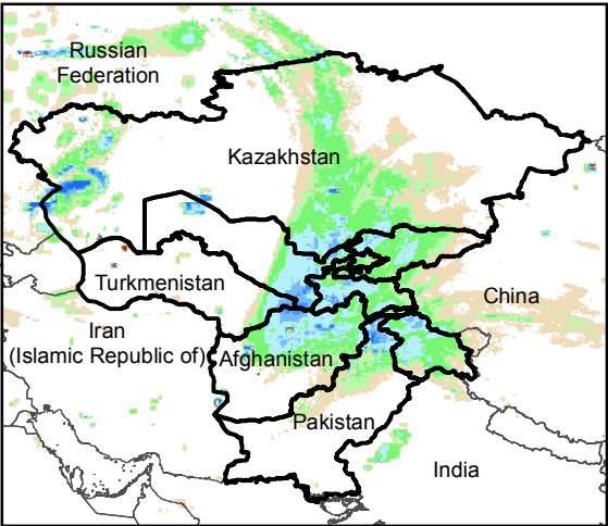
Daily Rainfall estimate for 4 Jan., 2016
