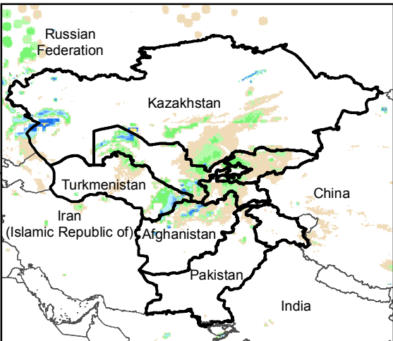
Daily Rainfall estimate for 7 Jan., 2016
