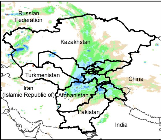
Daily Rainfall estimate for 7 Jan., 2016
