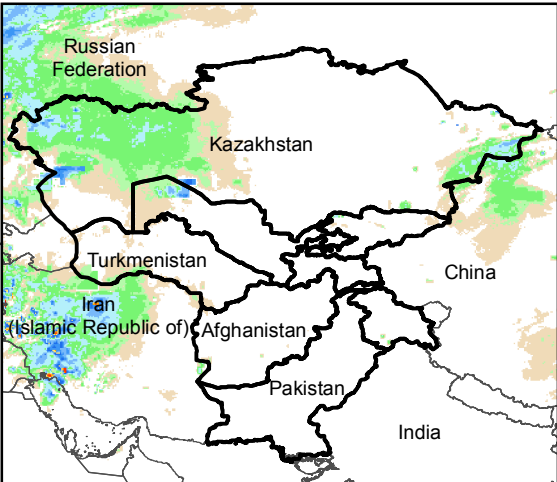
Daily Rainfall estimate for 9 Jan., 2016
