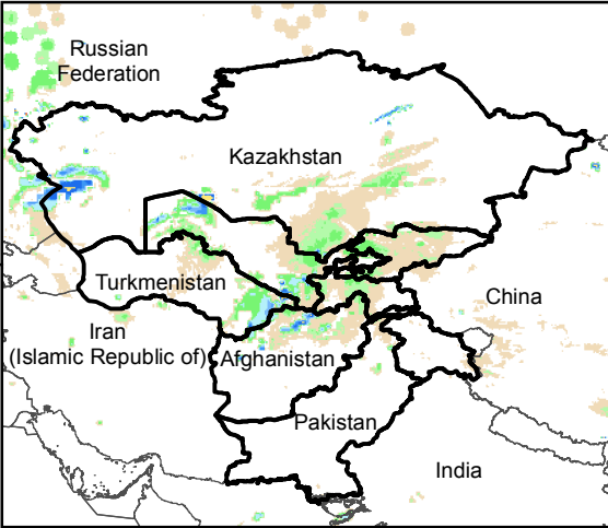
Daily Rainfall estimate for 10 Jan., 2016
