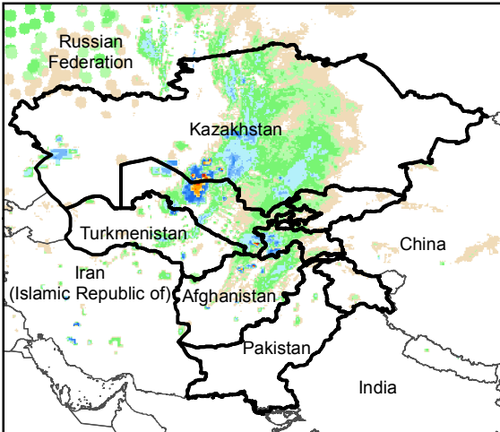
Daily Rainfall estimate for 11 Jan., 2016
