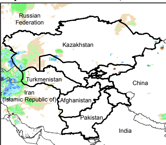
Daily Rainfall estimate for 24 Jan., 2016
