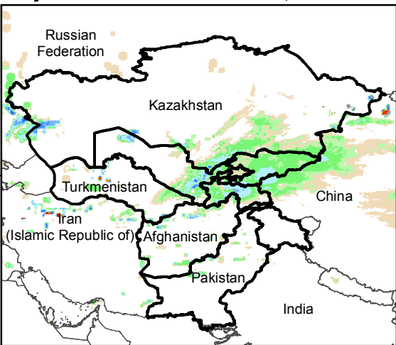
Daily Rainfall estimate for 31 Jan., 2016
