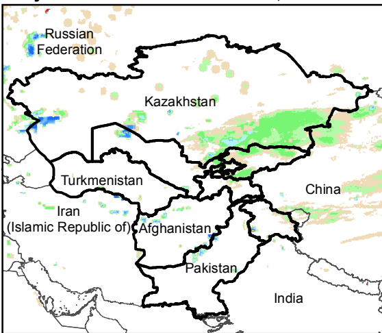
Daily Rainfall estimate for 3 Feb., 2016
