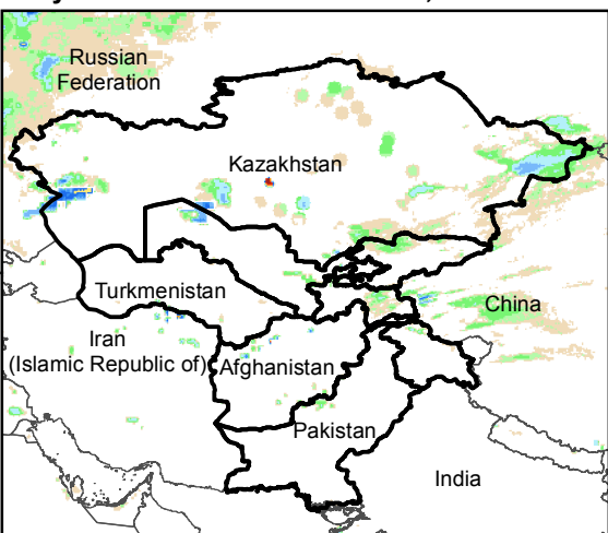
Daily Rainfall estimate for 1 Feb., 2016
