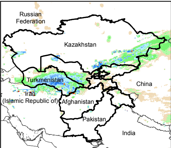
Daily Rainfall estimate for 9 Feb., 2016
