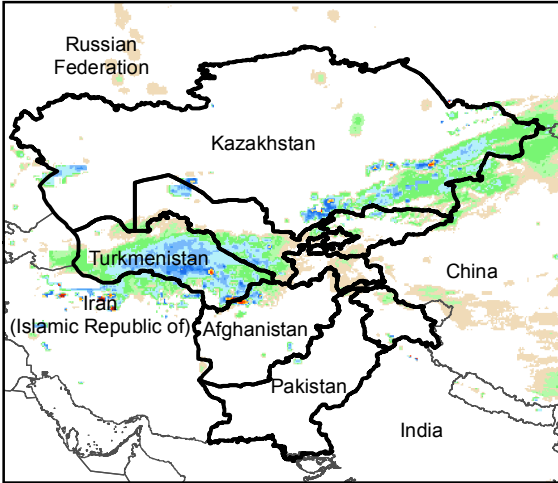
Daily Rainfall estimate for 12 Feb., 2016
