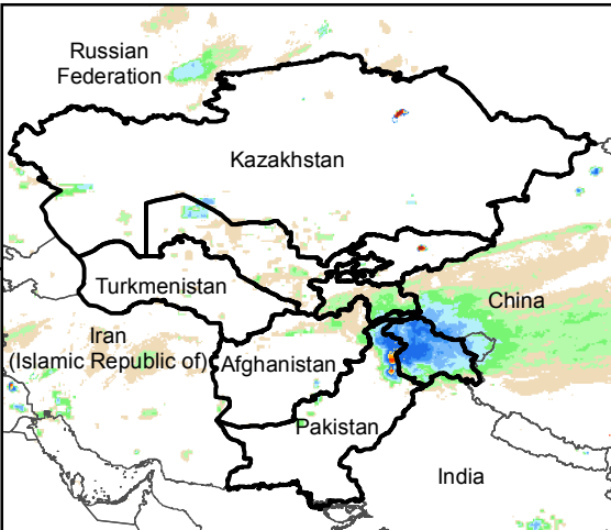
Daily Rainfall estimate for 11 Feb., 2016
