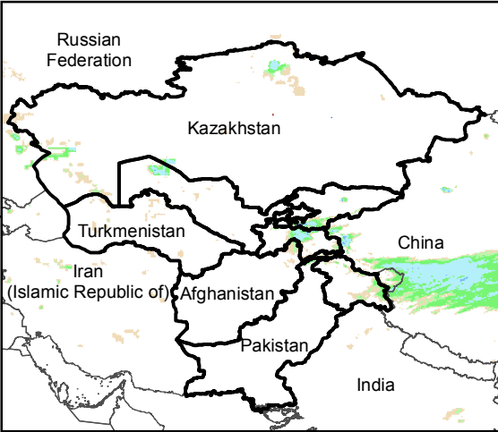
Daily Rainfall estimate for 16 Feb., 2016
