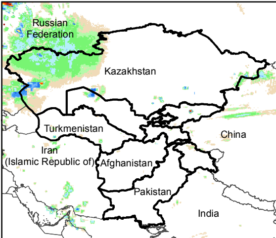
Daily Rainfall estimate for 17 Feb., 2016
