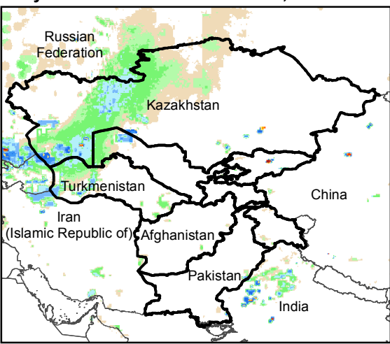
Daily Rainfall estimate for 18 Feb., 2016
