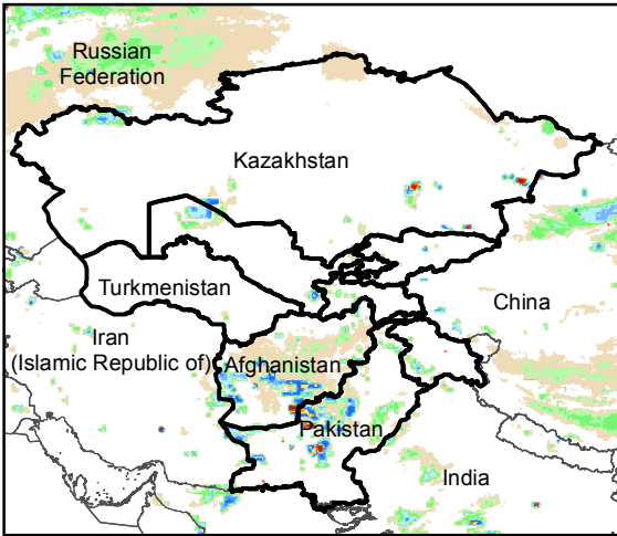
Daily Rainfall estimate for 6 Mar., 2016
