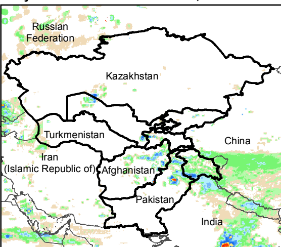
Daily Rainfall estimate for 6 Mar., 2016
