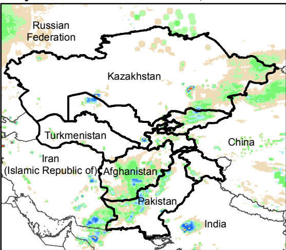
Daily Rainfall estimate for 5 Mar., 2016
