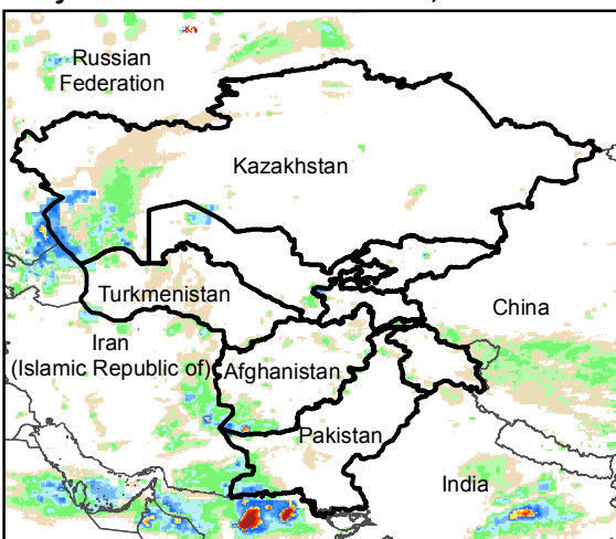
Daily Rainfall estimate for 7 Mar., 2016
