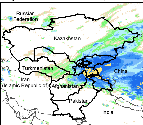
Daily Rainfall estimate for 18 Mar., 2016
