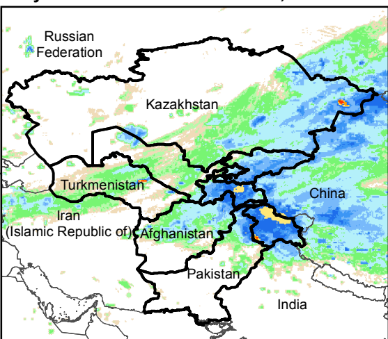
Daily Rainfall estimate for 17 Mar., 2016
