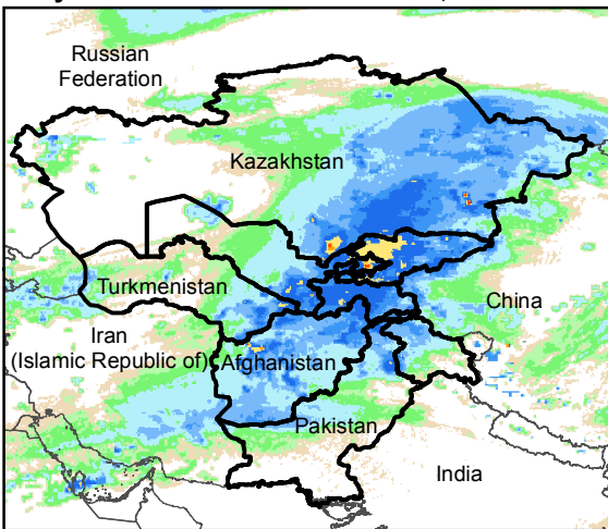
Daily Rainfall estimate for 19 Mar., 2016
