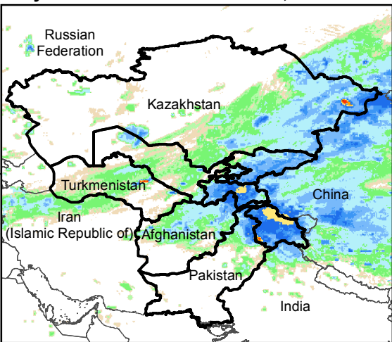
Daily Rainfall estimate for 20 Mar., 2016
