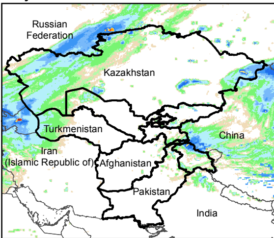
Daily Rainfall estimate for 23 Mar., 2016
