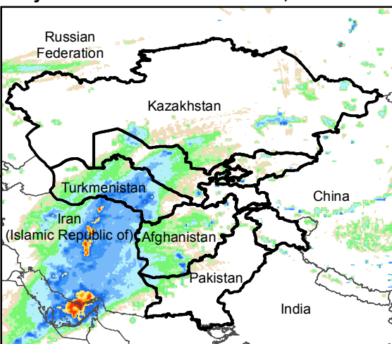
Daily Rainfall estimate for 22 Mar., 2016
