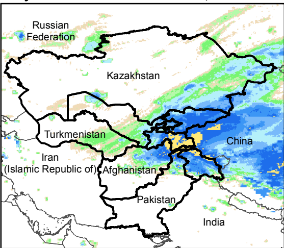
Daily Rainfall estimate for 21 Mar., 2016
