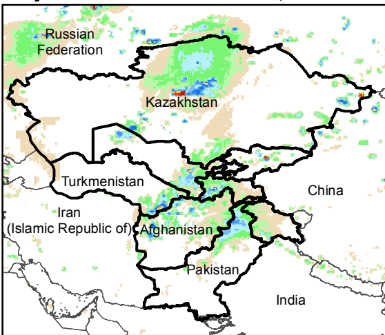
Daily Rainfall estimate for 27 Mar., 2016
