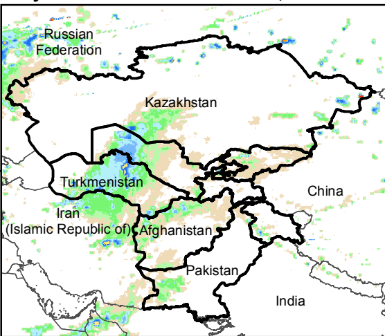
Daily Rainfall estimate for 26 Mar., 2016
