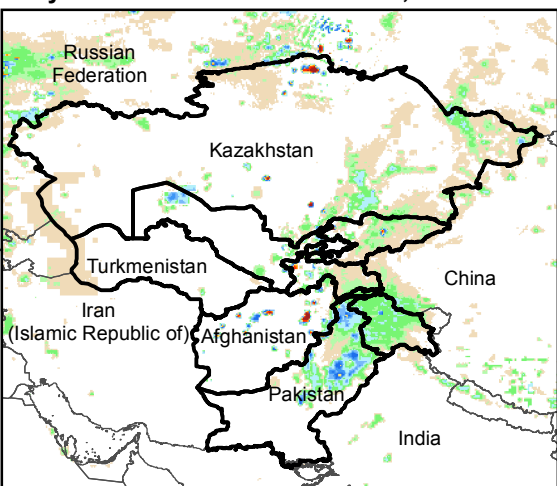
Daily Rainfall estimate for 25 Mar., 2016
