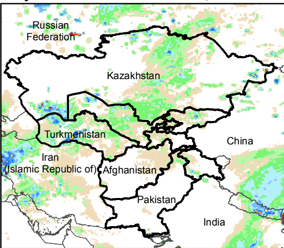
Daily Rainfall estimate for 31 Mar., 2016
