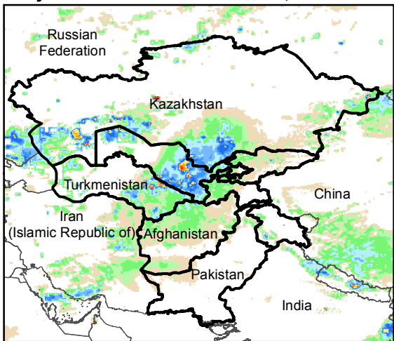
Daily Rainfall estimate for 2 Apr., 2016
