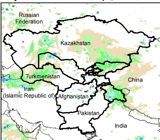
Daily Rainfall estimate for 4 Apr., 2016
