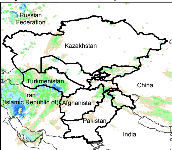
Daily Rainfall estimate for 18 Apr., 2016
