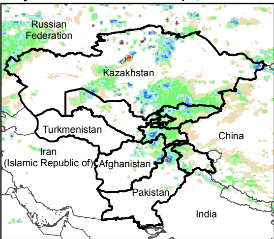
Daily Rainfall estimate for 24 Apr., 2016
