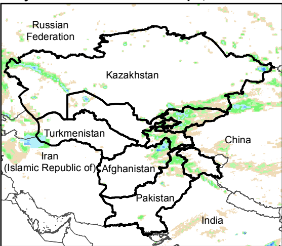
Daily Rainfall estimate for 29 Apr., 2016
