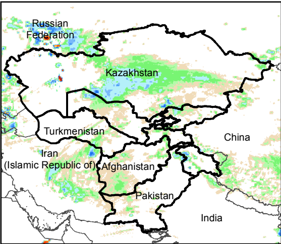
Daily Rainfall estimate for 1 May., 2016
