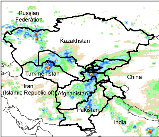
Daily Rainfall estimate for 3 May., 2016
