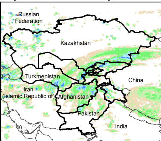
Daily Rainfall estimate for 5 May., 2016
