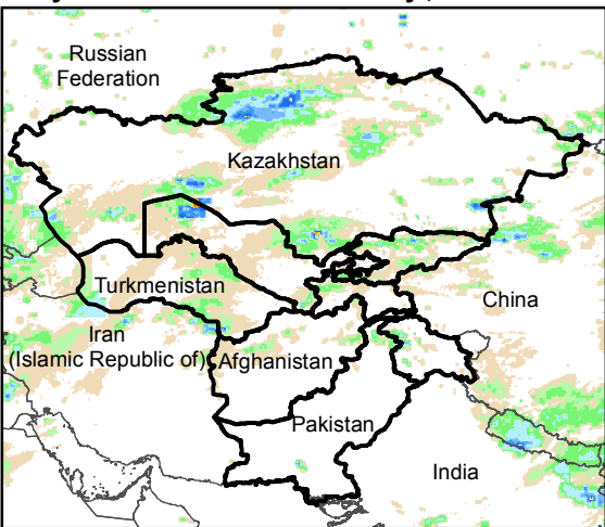
Daily Rainfall estimate for 10 May., 2016
