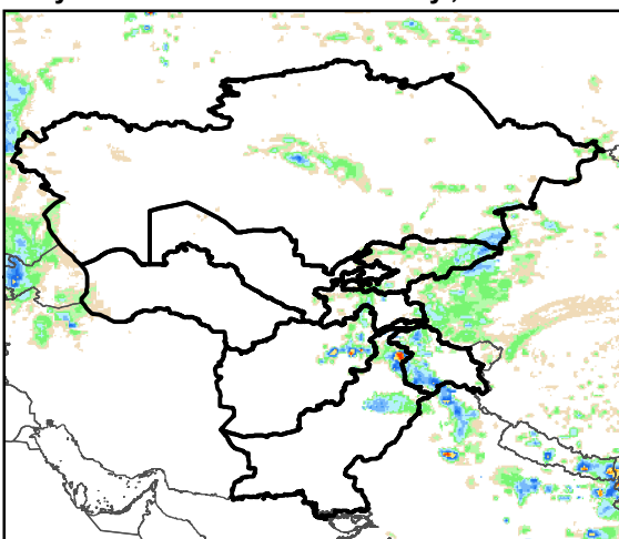
Daily Rainfall estimate for 24 May., 2016
