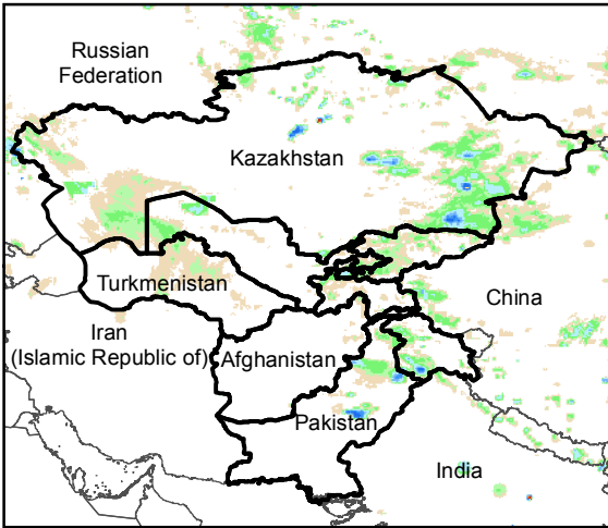
Daily Rainfall estimate for 29 May., 2016
