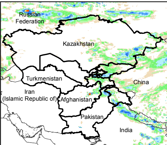
Daily Rainfall estimate for 28 May., 2016
