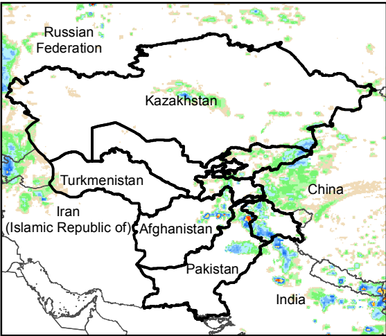
Daily Rainfall estimate for 27 May., 2016
