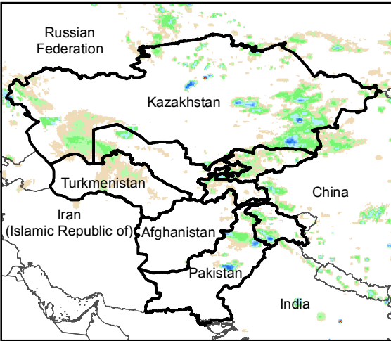
Daily Rainfall estimate for 29 May., 2016
