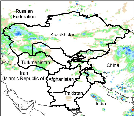
Daily Rainfall estimate for 31 May., 2016
