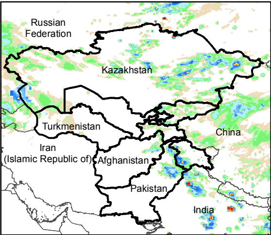
Daily Rainfall estimate for 30 May., 2016
