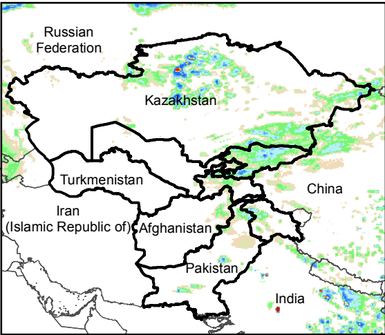
Daily Rainfall estimate for 30 May., 2016
