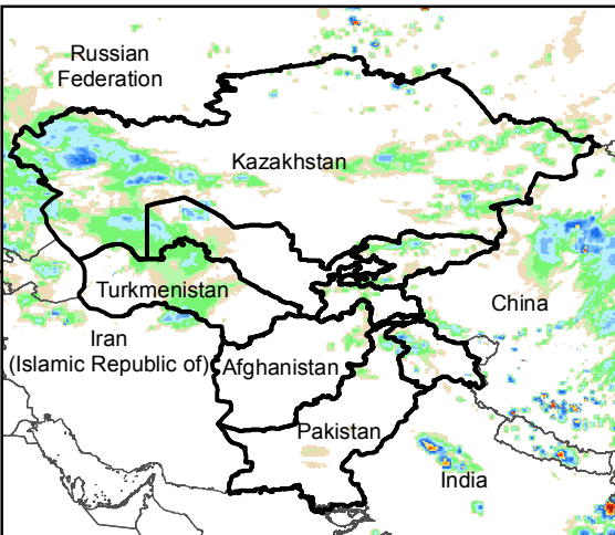
Daily Rainfall estimate for 31 May., 2016
