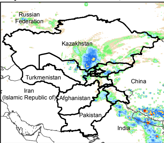
Daily Rainfall estimate for 18 Jun., 2016
