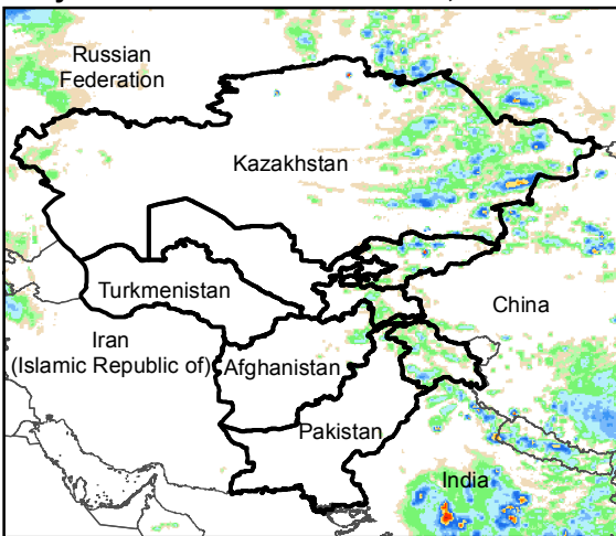
Daily Rainfall estimate for 21 Jun., 2016
