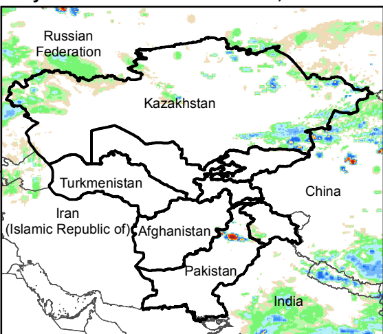
Daily Rainfall estimate for 19 Jun., 2016
