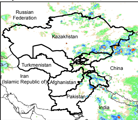
Daily Rainfall estimate for 20 Jun., 2016
