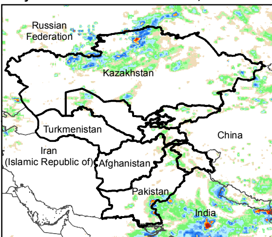
Daily Rainfall estimate for 25 Jun., 2016
