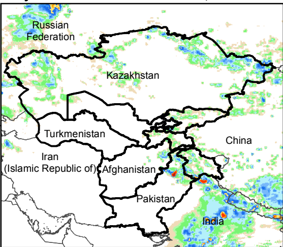
Daily Rainfall estimate for 23 Jun., 2016
