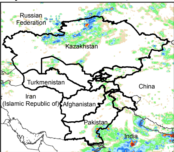
Daily Rainfall estimate for 28 Jun., 2016
