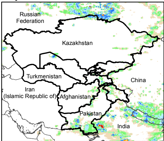
Daily Rainfall estimate for 3 Jul., 2016
