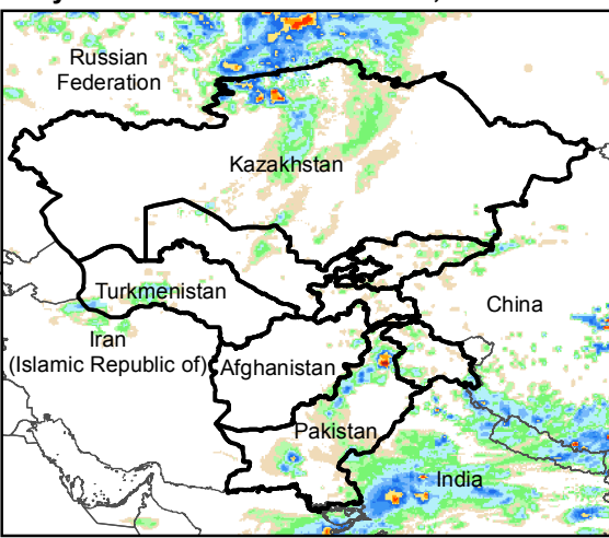
Daily Rainfall estimate for 13 Jul., 2016
