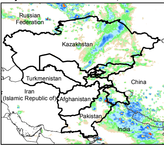
Daily Rainfall estimate for 14 Jul., 2016
