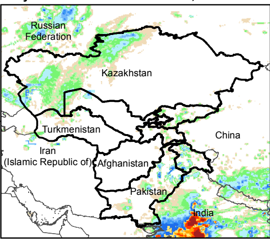
Daily Rainfall estimate for 12 Jul., 2016
