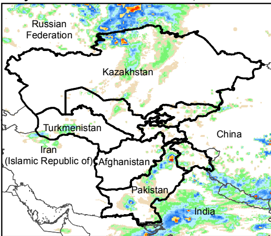
Daily Rainfall estimate for 16 Jul., 2016
