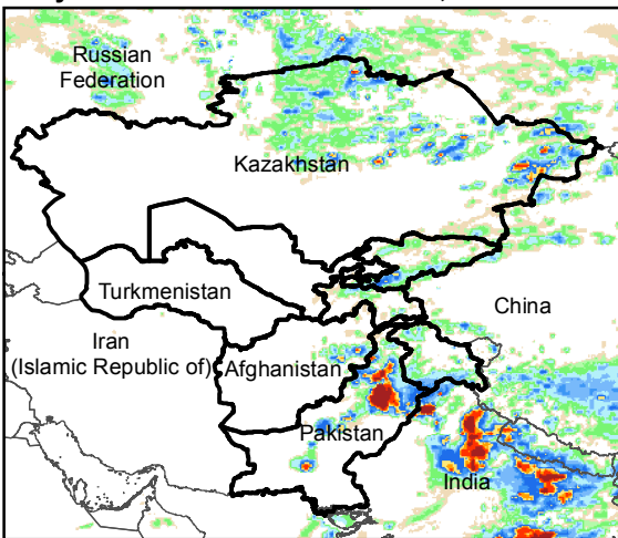
Daily Rainfall estimate for 20 Jul., 2016
