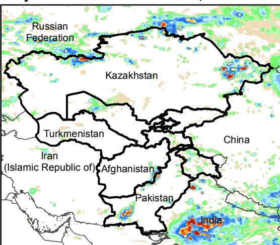
Daily Rainfall estimate for 24 Jul., 2016
