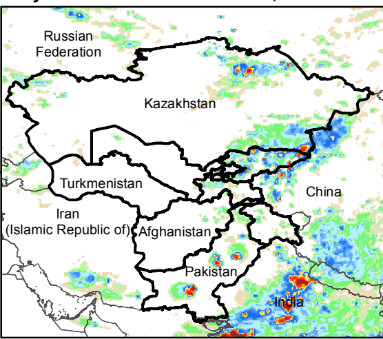
Daily Rainfall estimate for 31 Jul., 2016
