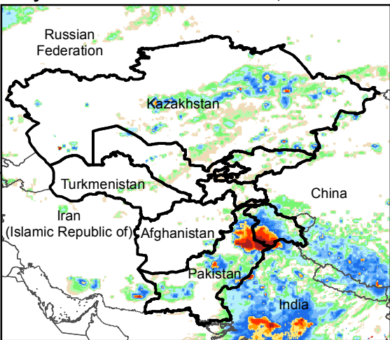
Daily Rainfall estimate for 30 Jul., 2016
