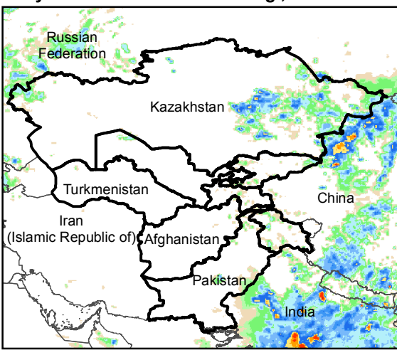
Daily Rainfall estimate for 1 Aug., 2016
