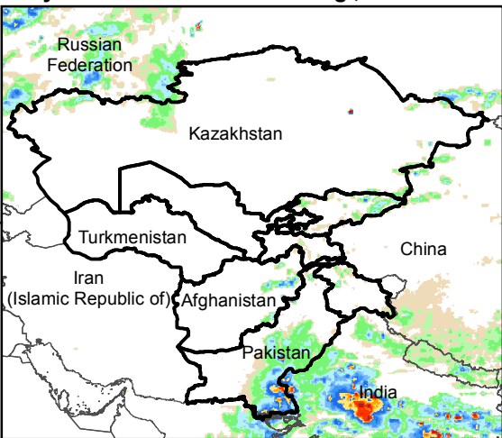
Daily Rainfall estimate for 7 Aug., 2016
